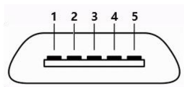
micro-USB 母头
